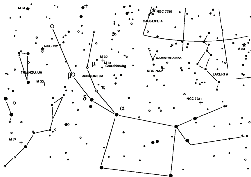
Fig. 16 Andromeda Galaxy
